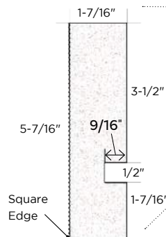
2X6 XT PLOWED FASCIA
